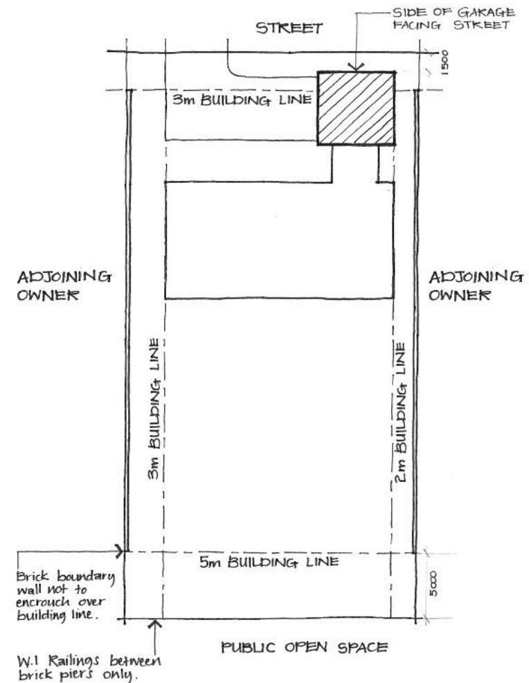
STREET INTERFACE B
