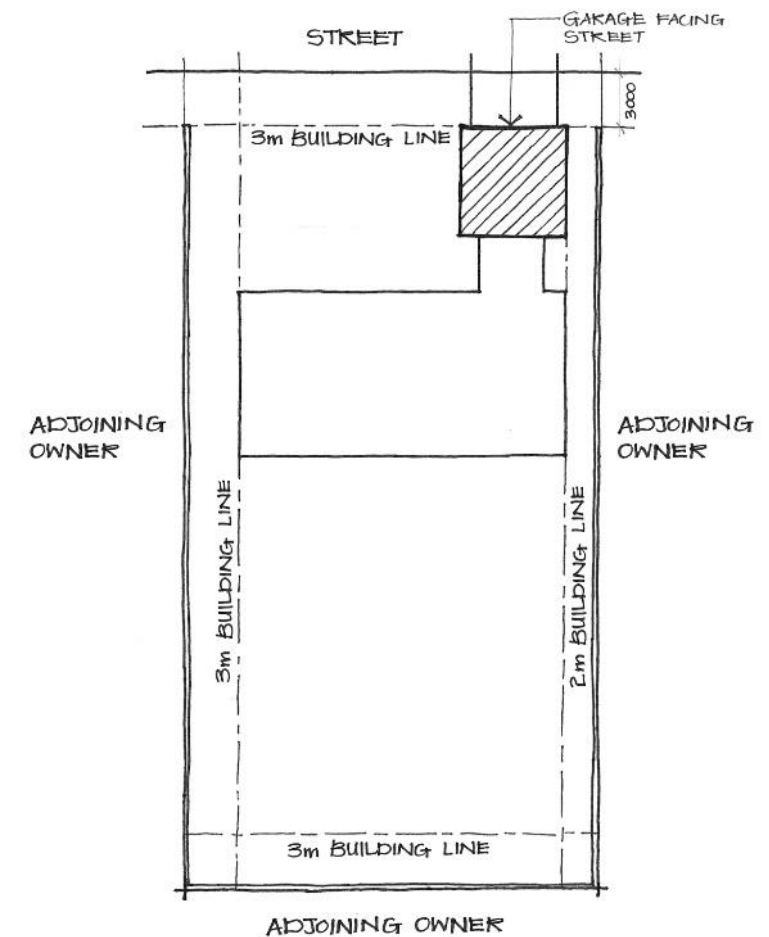
STREET INTERFACE A
